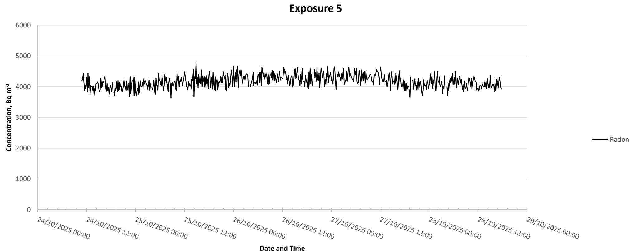
Figure 5. Radon concentration for exposure 5
