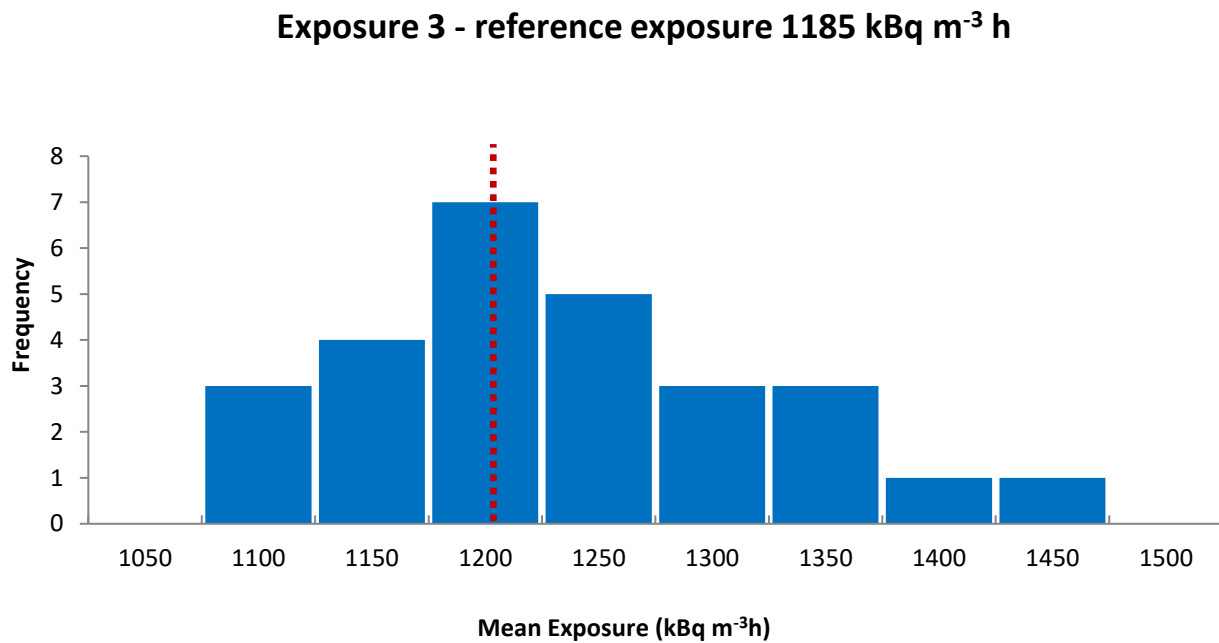
Figure 14. Distribution of mean exposure results for exposure 3 - given in Table 4.3 . The vertical dotted line indicates the reference exposure.
