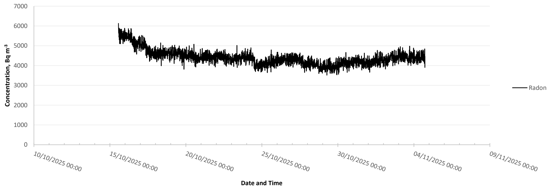
Figure 4. Radon concentration for exposure 4
